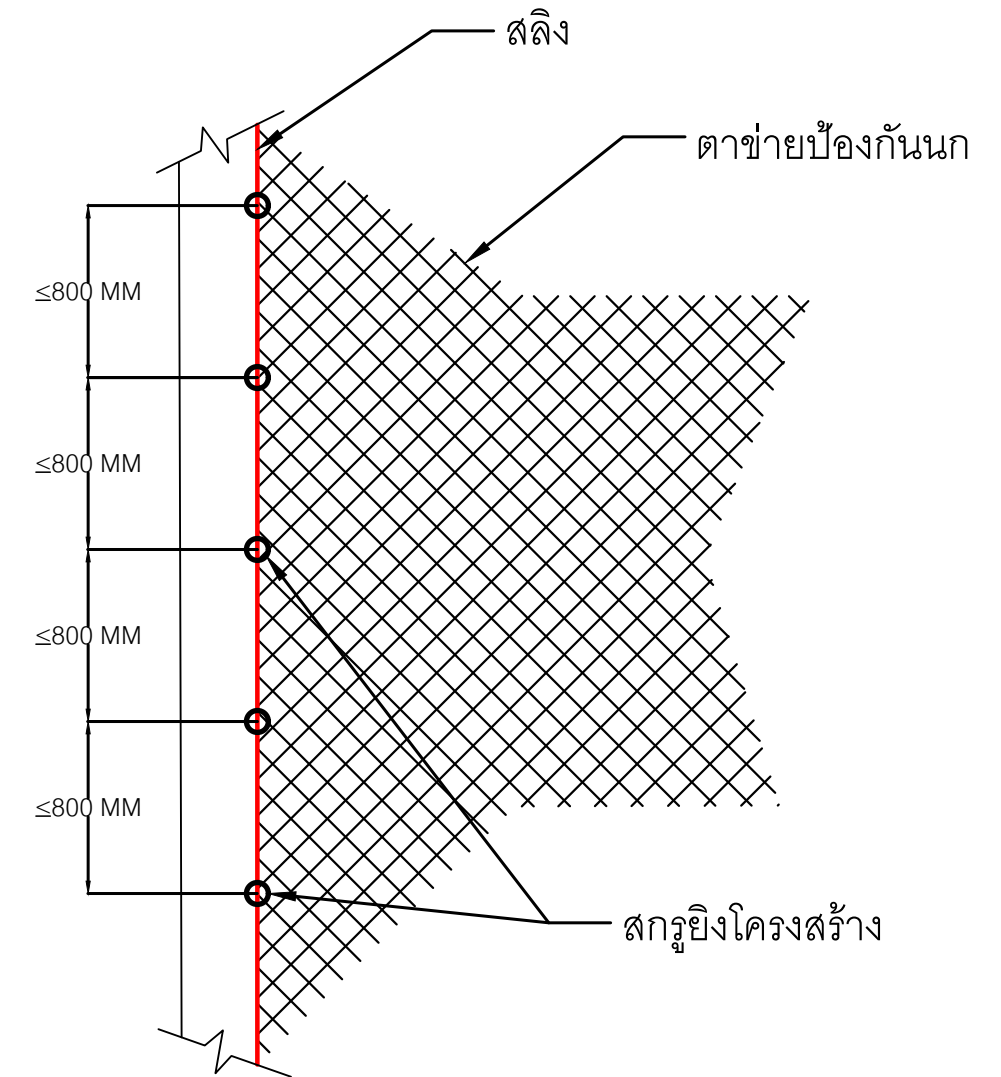
DETAIL A
